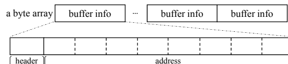
Figure 5: An illustration example for a byte array.
